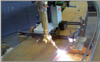
Auto Feed Plate Beveler
